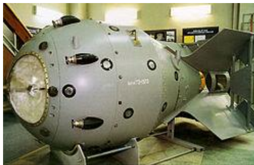
The first Soviet atomic bomb, "RDS-1", was an implosion type like the U.S. "Fat Man" bomb, even in appearance; the front "eyes" are radar fuses.
